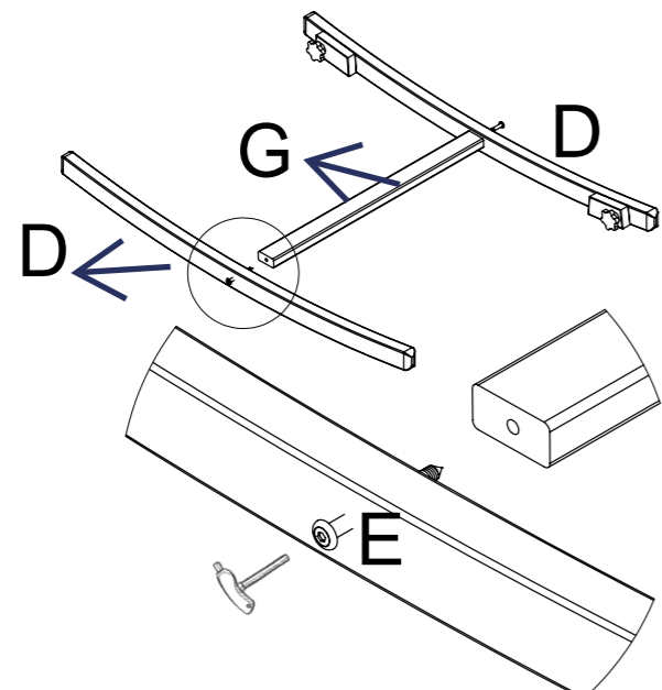
3.STEP
